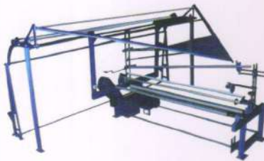
Double Fold Cum Rolling Machine
